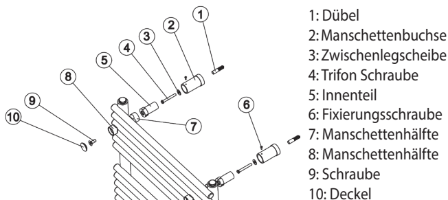
Figure 5: Assembly Parts
